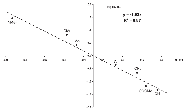
Fig. 2 Hammett plot obtained from competition experiments using a series of para -substituted anilines.
